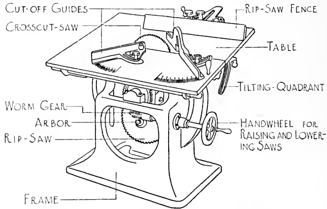
FIG. 156. UNIVERSAL CIRCULAR SAW TABLE.
